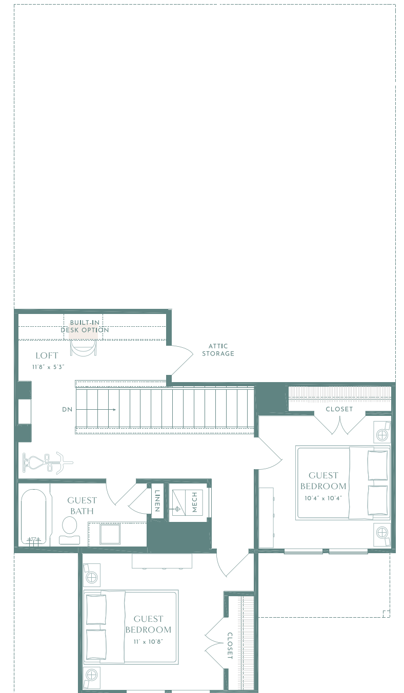
LEVEL 2
